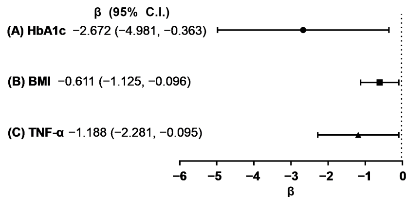
Figure 3. Beta-coefficient ( \beta ) and 95% confidence intervals (C.I.) from multiple linear regression with HbA1c (A), BMI (B), TNF- \alpha (C), and vitamin D as outcomes in women.
